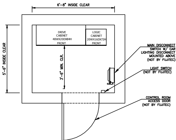
CONTROL ROOM - HVF
