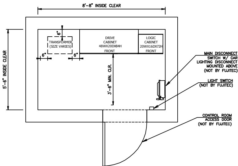
CONTROL ROOM - HVF W/ TRANSFORMER
